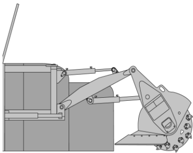
SG60 and SGX60 Stump Grinder
